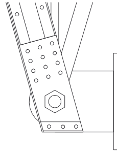
End Connection
